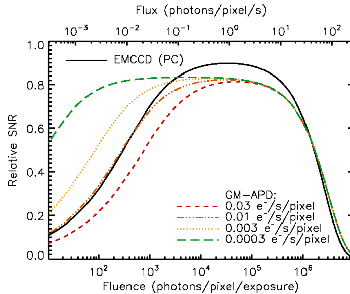
Figure 9. This plot shows relative SNR (normalized to \sqrt{\text{Fluence}} ) for a state-of-the-art EMCCD and GM-APDs with various values for dark count rate. The current state-of-the-art DCR for the GM-APD is shown, as well as 1/3, 1/10, and 1/100 reduction in DCR. For even the 1/3 reduction in DCR, the GM-APD is comparable to EMCCD performance due to the clock-induced-charge that plagues the EMCCD.
