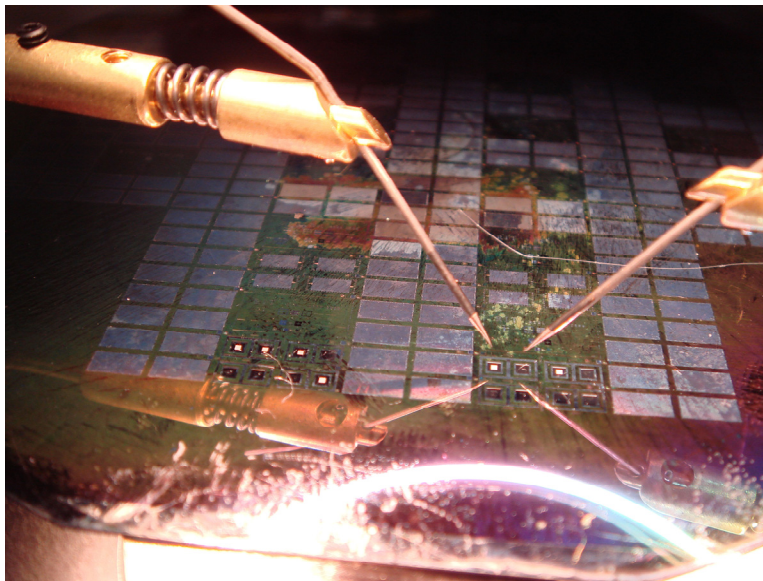
Figure 24. This image is a close-up of a device wafer being tested on the probe station.
