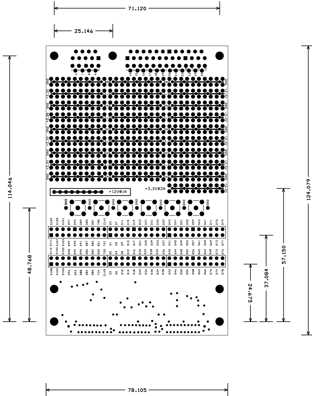
HSMC PROTOTYPE BOARD MECHANICAL DIMENSIONS IN MM
