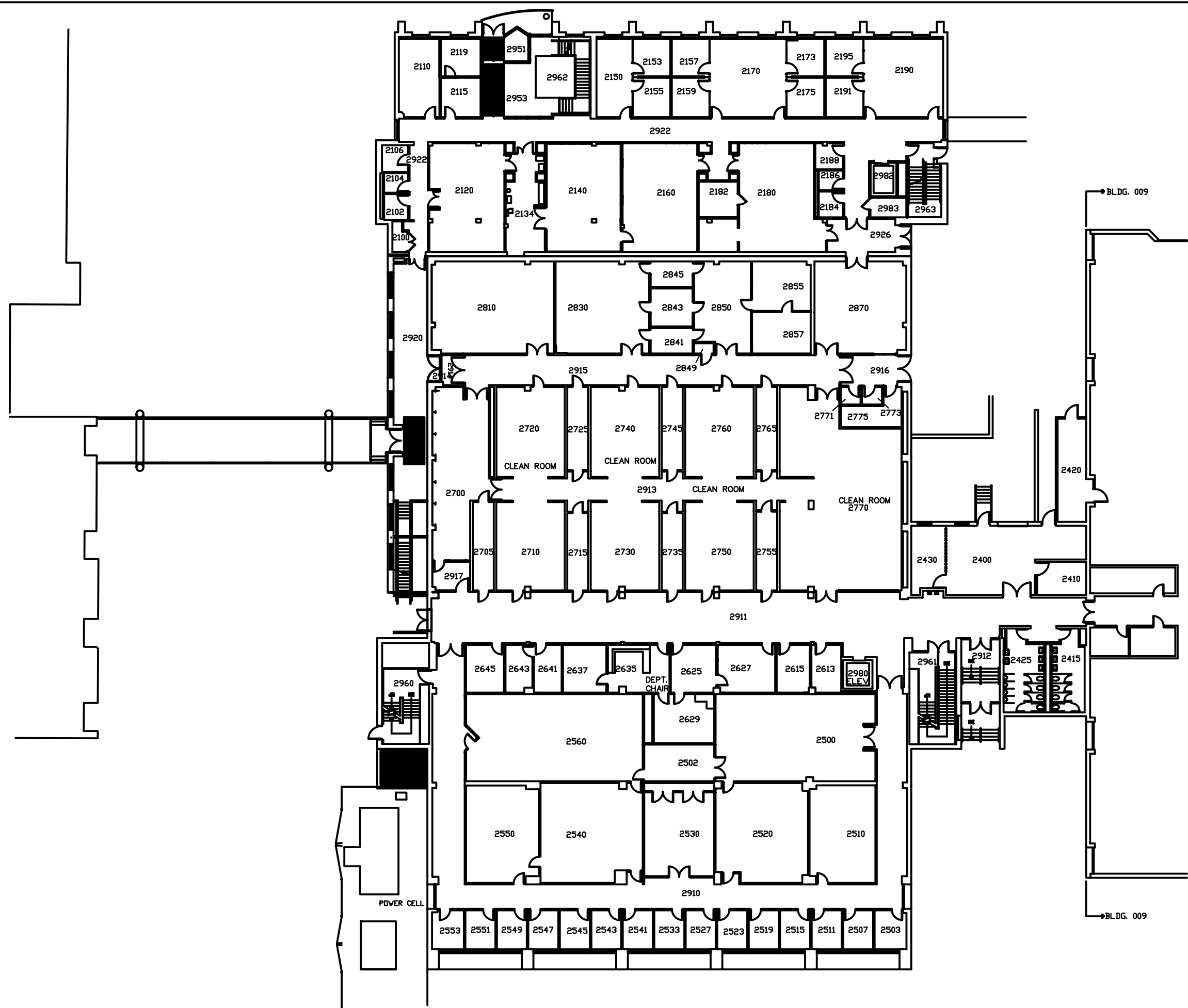
Bldg 017 Microelectronics Bldg. Second Floor Plan
