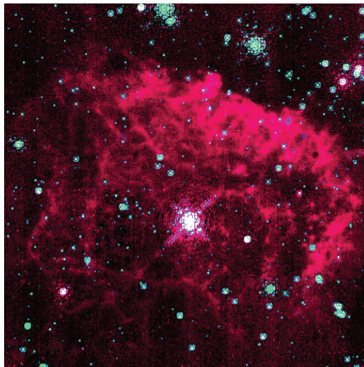
The Pistol Star
